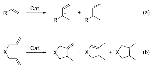
Scheme 1. (a) Hydrovinylation of olefins (R = Ar, for example) and (b) cycloisomerisation of 1,6-dienes [X = C(CO 2 R) 2 , N–R, O, for example].
