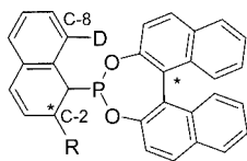
Scheme 2. The quinaphos ligand family with \beta -binaphthol as the diol moiety ( D = \text{Cl}, \text{OMe}, \text{PPh}_2 ; R = \text{alkyl or aryl, for example} ).
