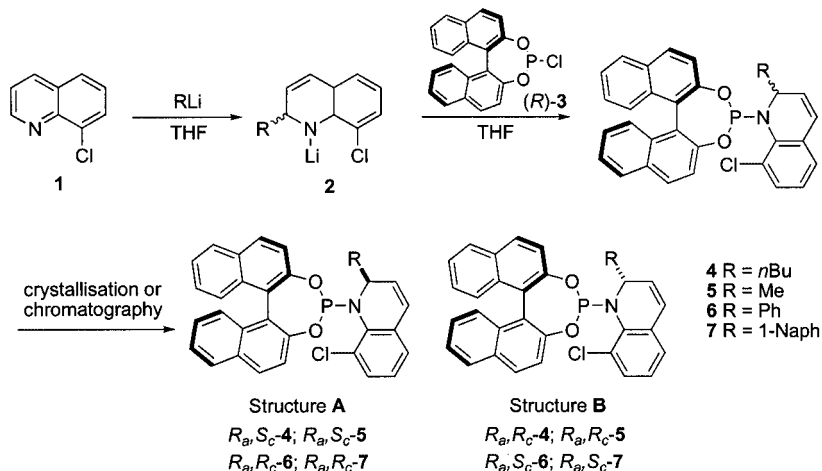
Scheme 3. Synthesis of monodentate quinaphos phosphoramidites.
