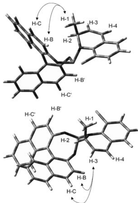
Figure 2. Calculated conformational minima of ( R a ,S c )- 5 (top) and ( R a ,R c )- 5 (bottom). The arrows show selected NOE interactions.
