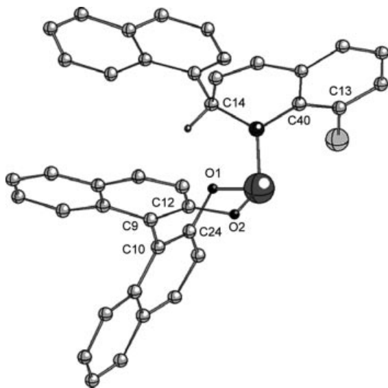
Figure 1. ORTEP of ( R a ,S c )- 7 .
